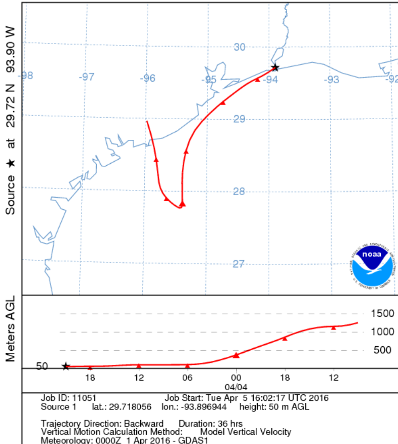
NOAA HYSPLIT MODEL Backward trajectory ending at 2100 UTC 04 Apr 16 GDAS Meteorological Data
